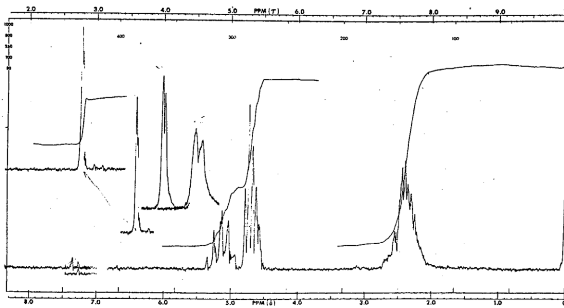
Figure IX: N.M.R. Spectrum of 4,5-hexadienal Sweep offset = 150 cps.
